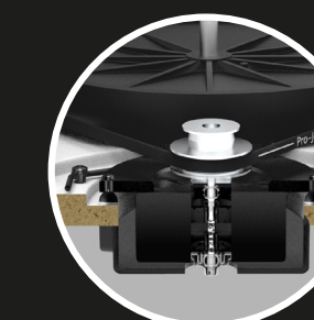
Silicon-damped Motor Suspension
